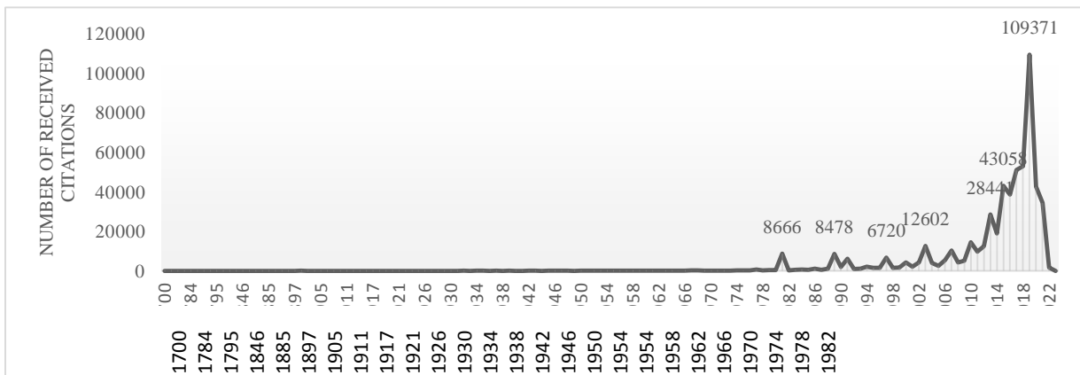
Figure 6. RPYS Analysis of the Third Period
