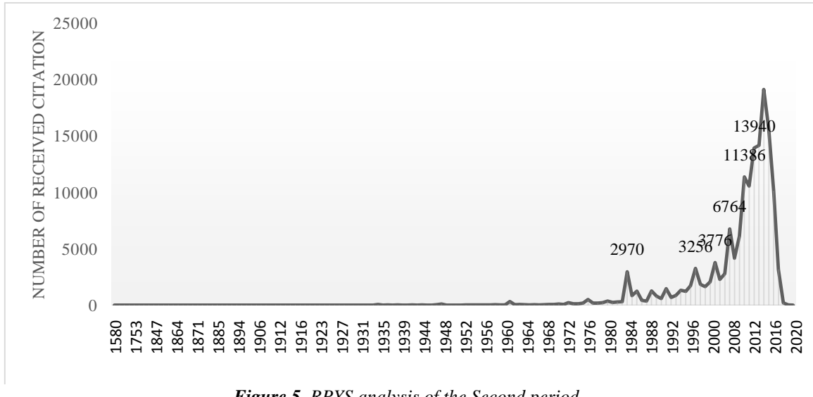
Figure 5. RPYS analysis of the Second period
